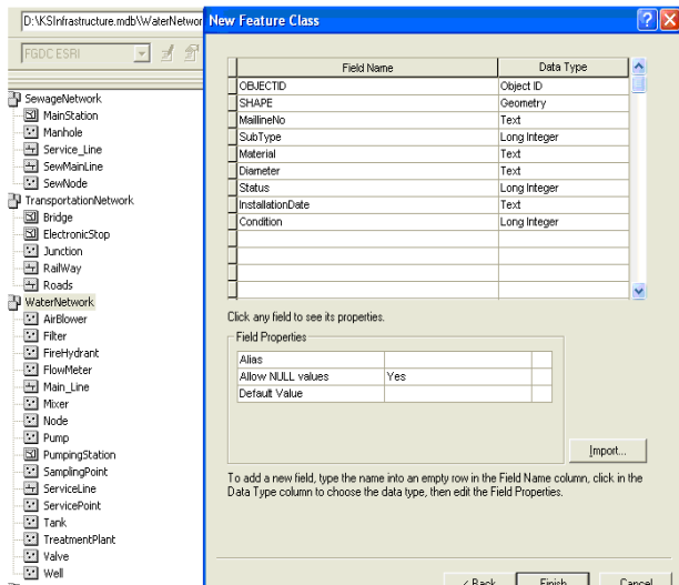
Fig. 10 The feature classes
