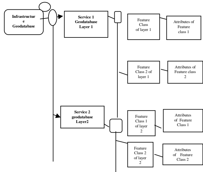
Fig. 3 The Navigation of the proposed Infrastructure Ontology layers
